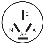
4 pin plug socket connection
