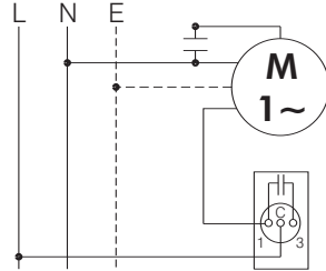
SSC - 2 SPEED SWITCH
