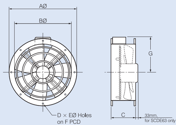
Dimensions, mm
